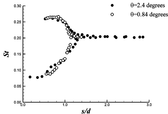
Fig. 11. Spanwise variation of vortex shedding frequency (non-parallel pair of circular cylinders, \theta = 2.4^\circ and 0.84^\circ ).
